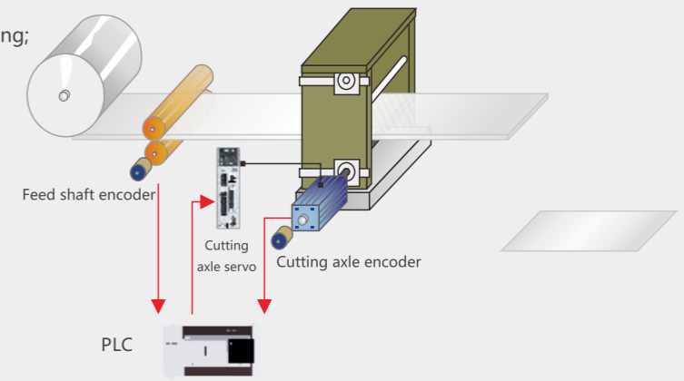
E-cam -- Flying shear function
