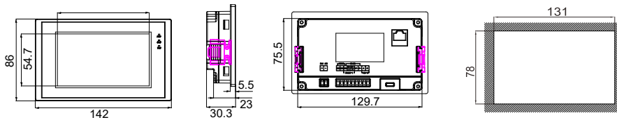
PI3043ieS / PI3043ieS-N installation size
