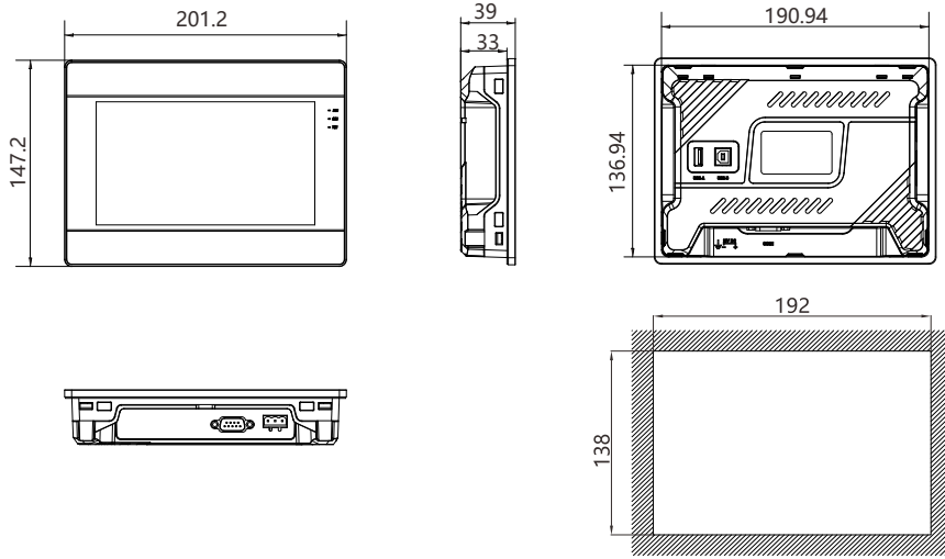
PI2070ie / PI3070ie installation size
