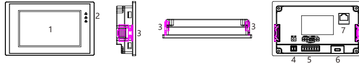
PI3043ie / PI3043ie-N Components description
