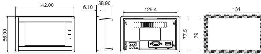
PI3043ie-T installation size
