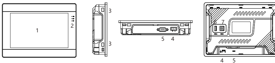
PI2070ie / PI3070ie Components description
