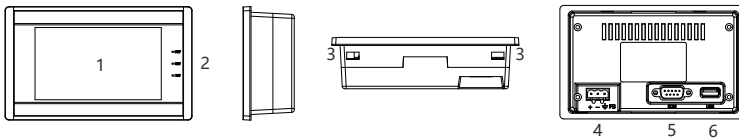
PI3043ie-T Components description
