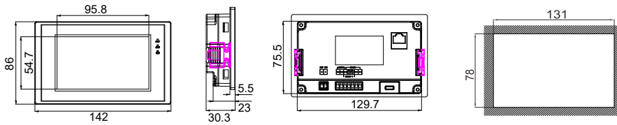
PI3043ie / PI3043ie-N installation size
