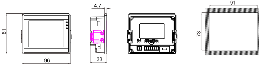
PI3035ie installation size
