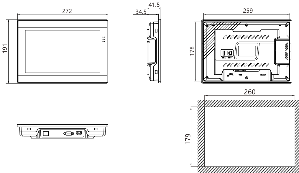
PI2102ie / PI3102ie installation size
